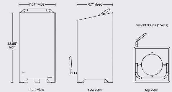
LiteWare RGB Battery Uplighter dimensions
